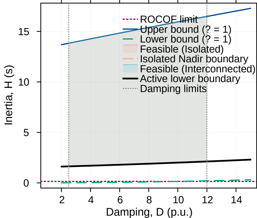
Area 1 frequency-security region
