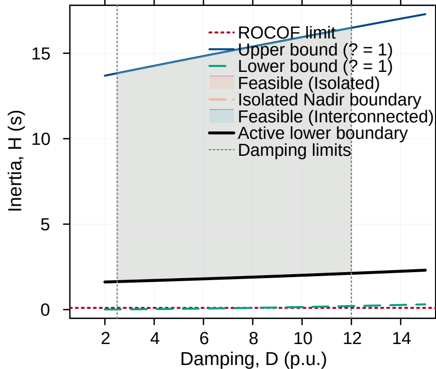
Area 2 frequency-security region
